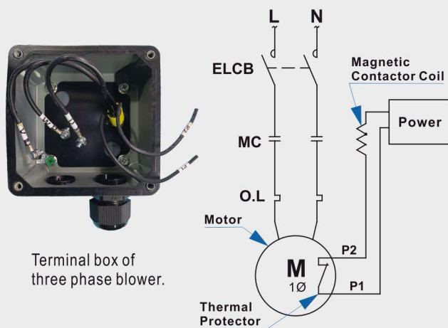
P1,P2 wiring diagram for three phase blower.
