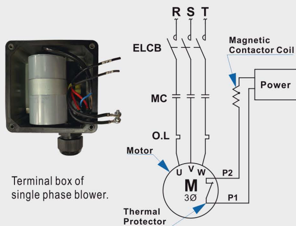
P1,P2 wiring diagram for single phase blower.
